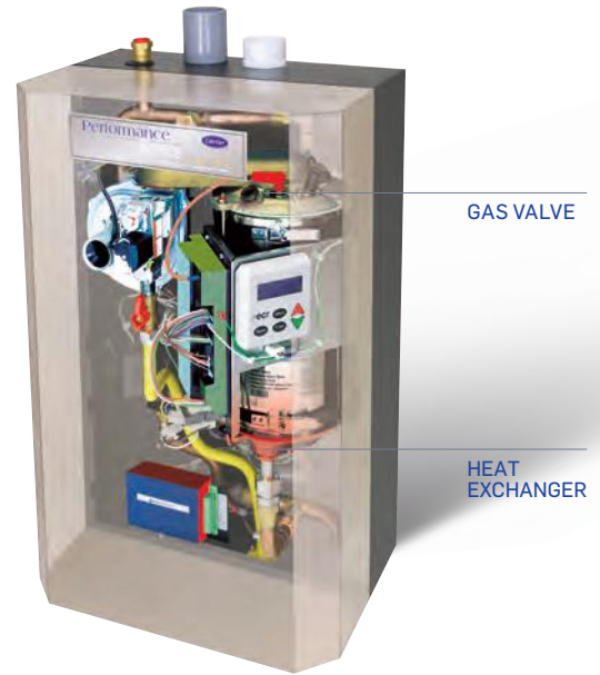
PERFORMANCE 95 BOILER MODEL BWM SHOWN
